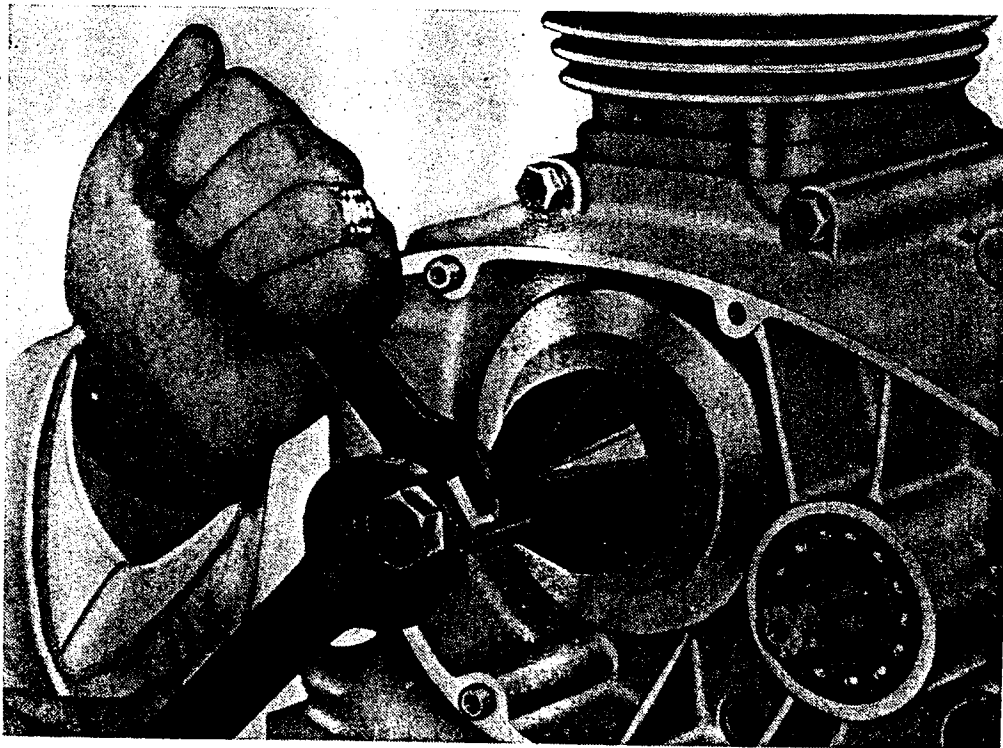
1 - Flywheel puller
